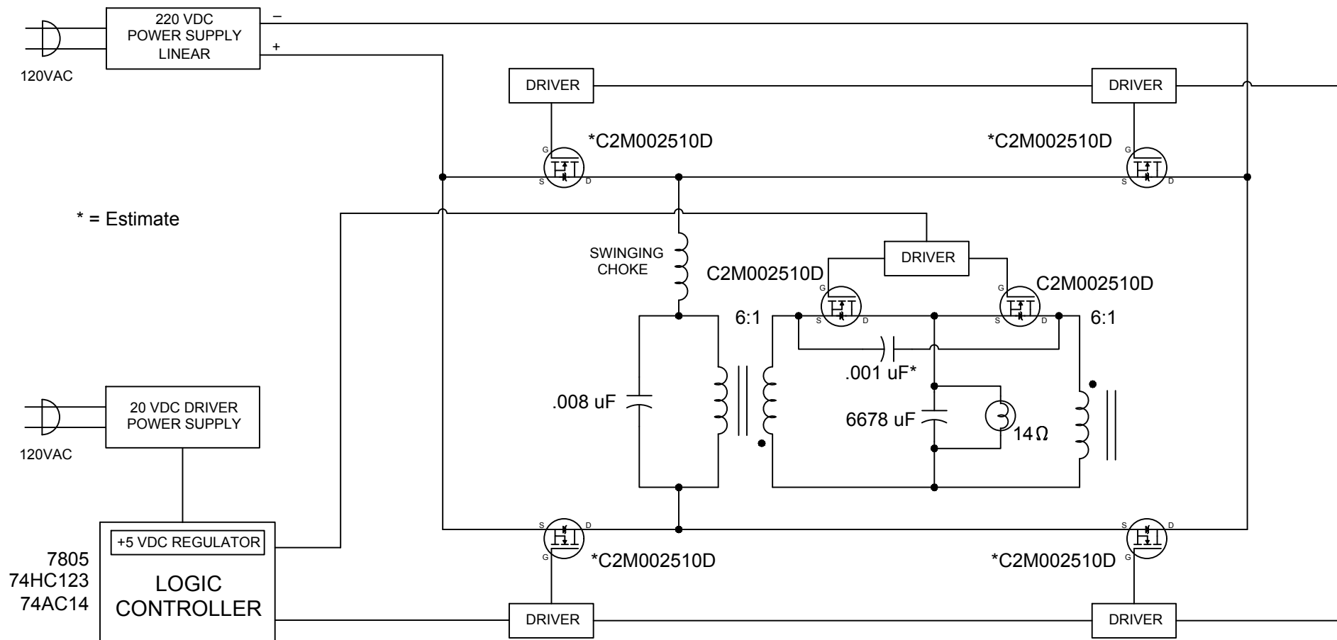
Graham Gunderson Overall System Schematic Presentation Version drafted 8/4/2016 by Mark McKay
