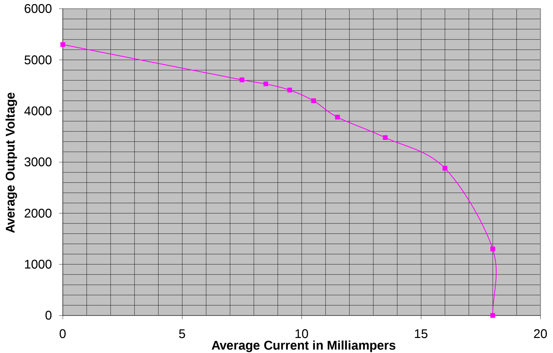
12 - 5000 Volt Inverter Performance
