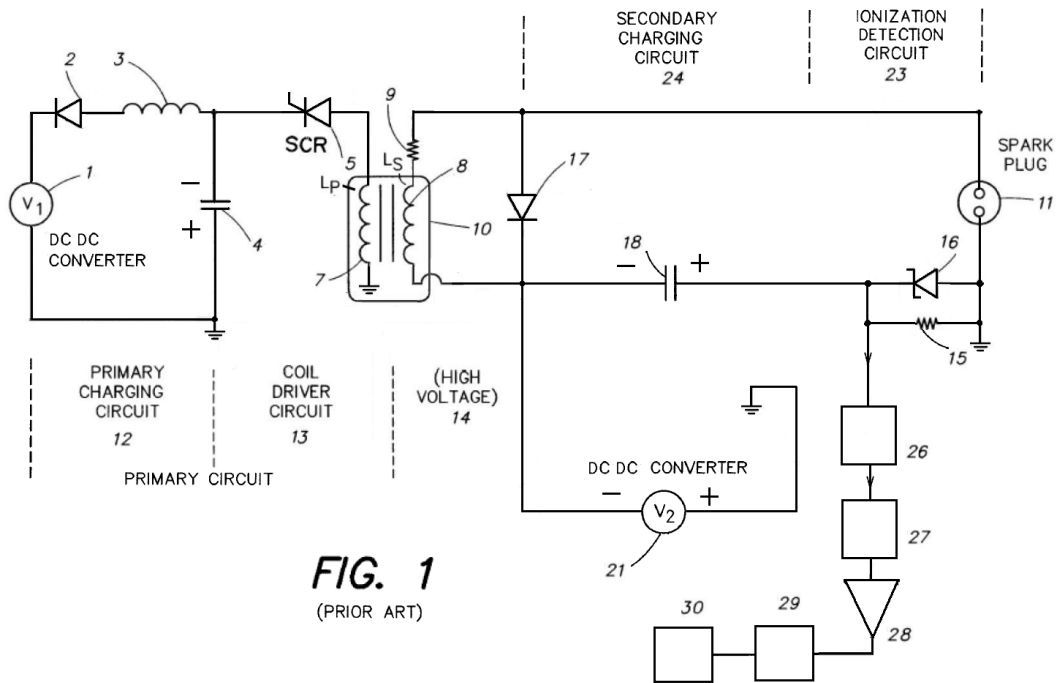
Figure 1: Dual Energy Ignition System with ionization detection (disclosed in U.S. Pat. No. 5777216 to Van Duyne et al)
